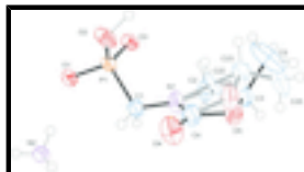
Fig. 1. The asymmetric unit of title compound with the atom numbering scheme showing 50% probability displacement ellipsoids. H atoms are shown as small spheres of arbitrary radii. Minor occupancy disorder component is represented with dashed lines.
